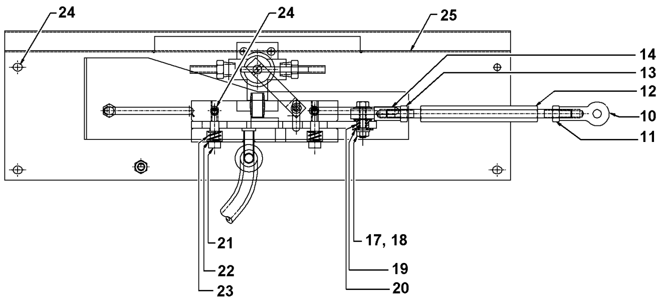
Pull Guide Drive Assembly (Viewed at N.O.S.)
