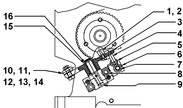
Pull Guide Drive Assembly (Viewed at N.O.S.)
